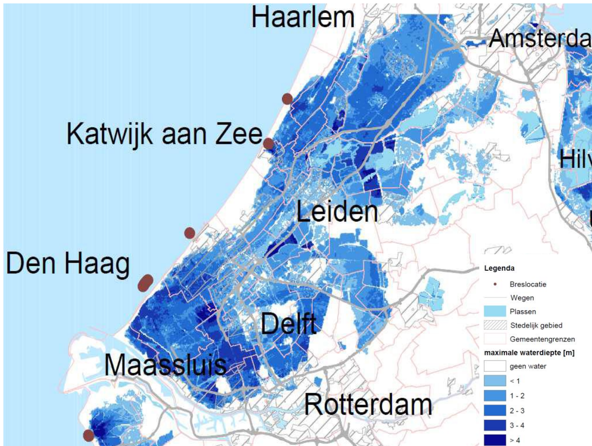
Figure 3-4: Worst case case scenario North Sea; source: Coördinatieplan dijkkring 14, RWS
