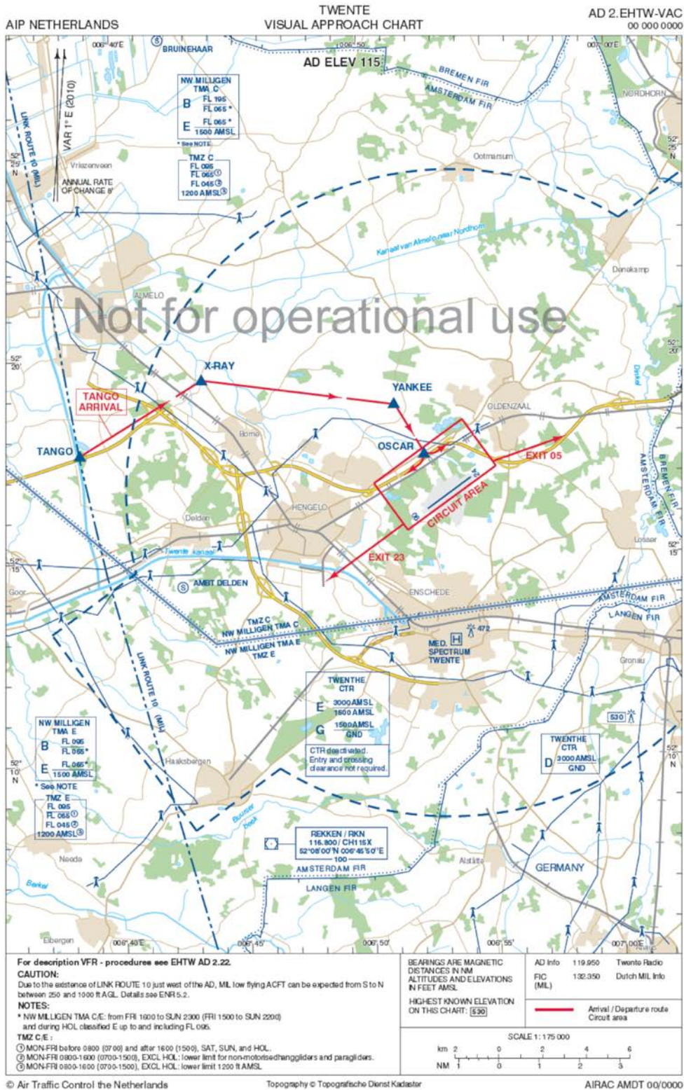
Figur 2-2: Concept Visual Approach Chart Twente
