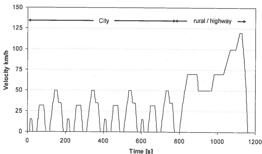
Figure 2: NEDC (New European Driving Cycle).
