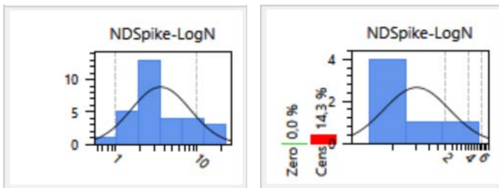
Figure 3. Example of a 'NonDetectSpike LogNormal' distribution fitted to the MOSH concentrations of the food group 'chocolate' (A) (0% non-detect samples) and 'breakfast cereals' (B) (14% non-detect samples)
