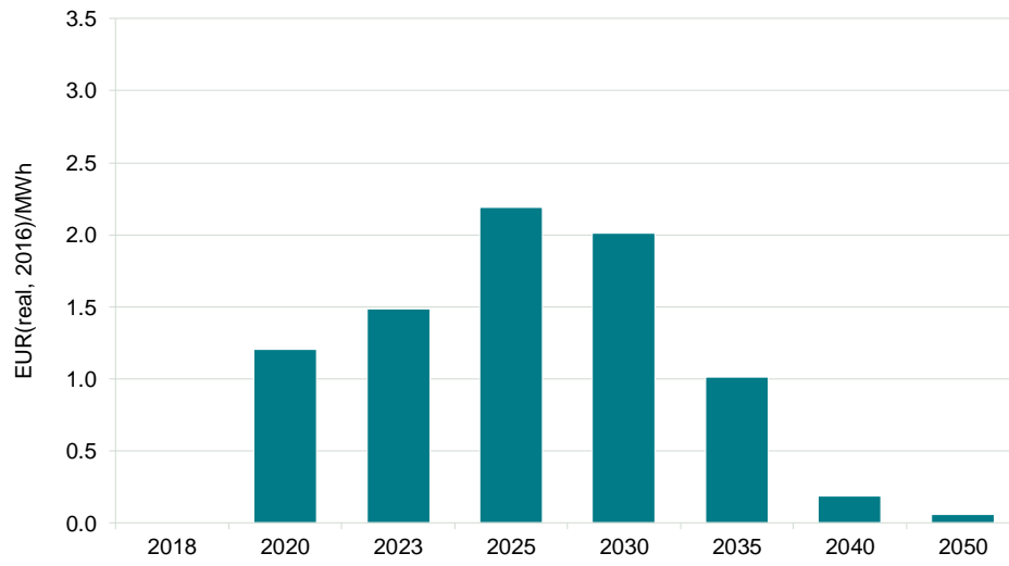
Figure 30 CPF – Impact on power prices
