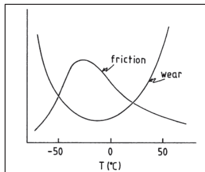
Figure 3.4: Relation of friction and wear versus temperature of a rubber compound [12].
