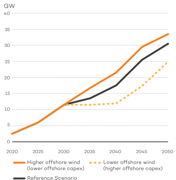
FIGURE 21 – INSTALLED CAPACITIES OF OFFSHORE WIND (GW) IN THE NETHERLANDS FOR HIGH WIND SENSITIVITIES
