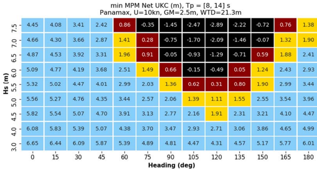
Minimum dynamic UKC in waves, GM=2.5m for speed of 10 knots.
