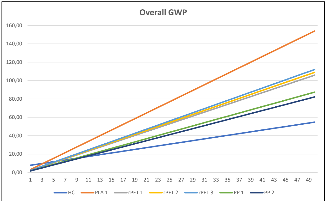
Figure 25: Graph of Overall GWP for Hard and Soft Cups
