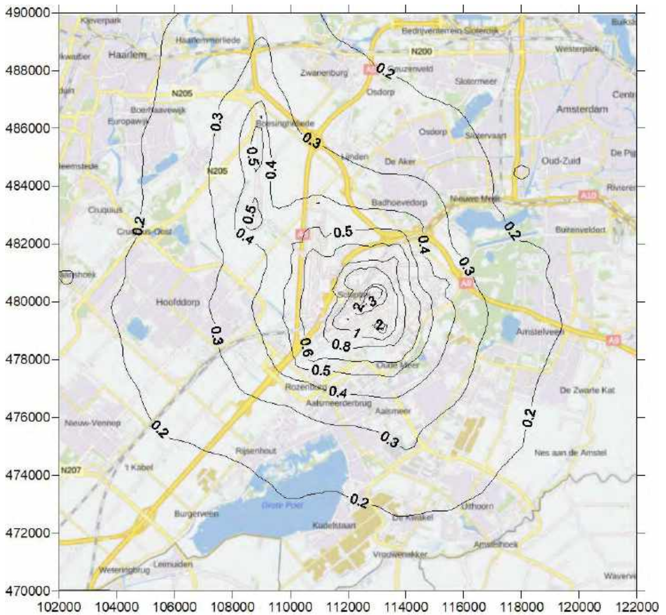
Figuur K.46: Contourplot (20 x 20 km) van de 98 percentiel VOS scenario 450k_NNHS (2020) in \text{ouE}/\text{m}^3
