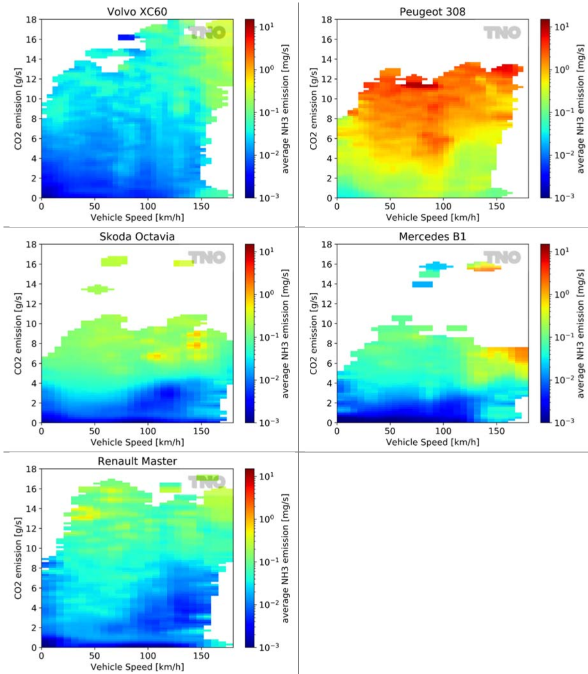
Figure 4-3: Two-dimensional emission map of average NH 3 emissions shown dependent on CO 2 emissions and vehicle speed.
