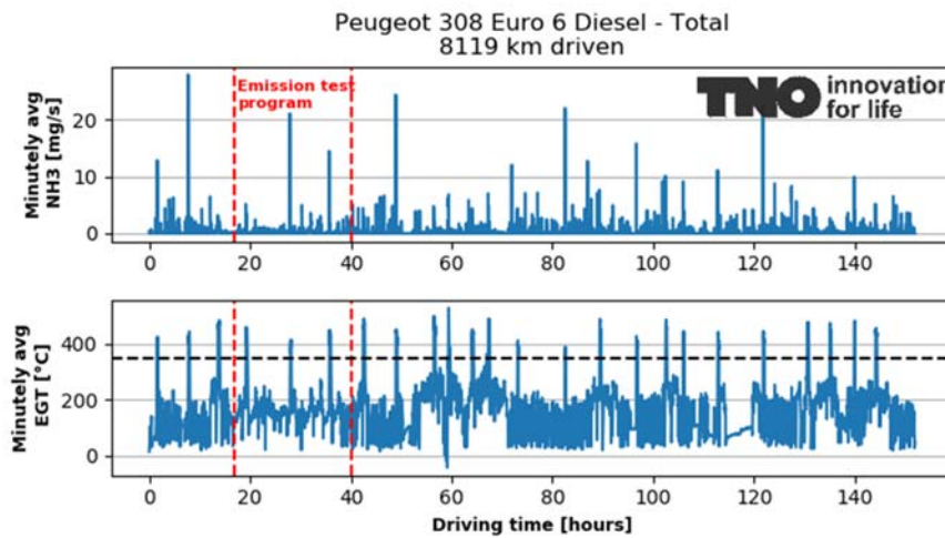
Figure A-16: NH 3 emission and exhaust gas temperatures over the test programme (in total 151.9 hours) of the Peugeot 308. The red dotted lines mark the period of the emission test program.
