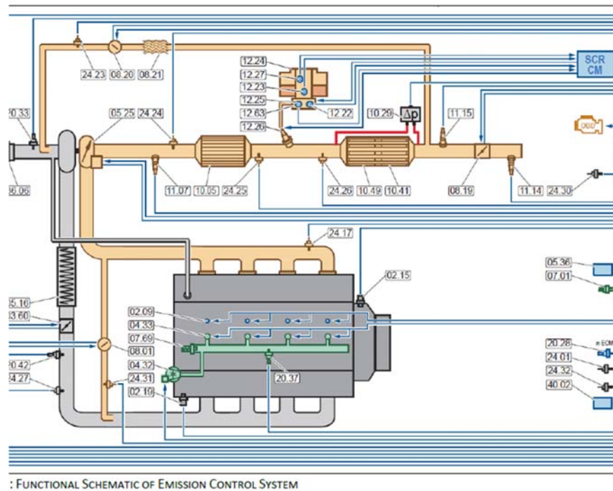
Figure A-38: Functional schematic of the Mercedes B180's emission control system (source: Mercedes-Benz Cars Nederland B.V).
