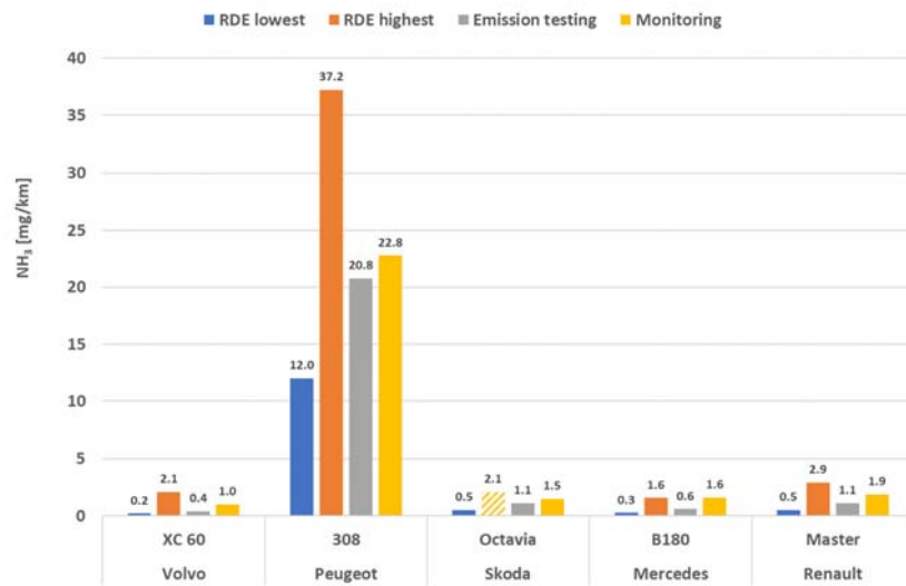
Figure A-60: NH 3 test results of 'RDE' tests, the emission test programme and the monitoring programme of the five tested Euro 6d-Temp diesel vehicles.
