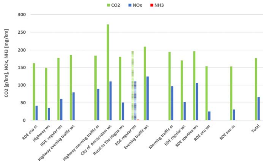
Figure A-13: Average CO 2 , NO x and NH 3 results of the emission test programme of the Volvo XC 60.
