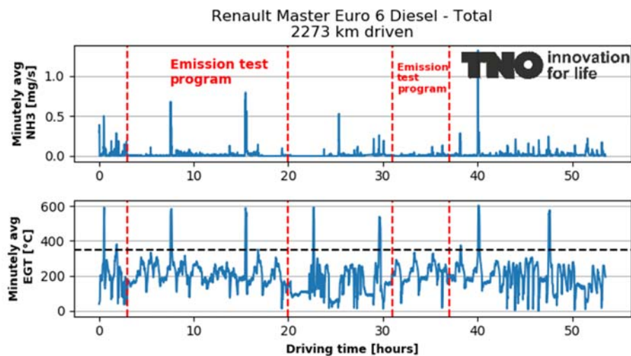
Figure A-48: NH 3 emission and exhaust gas temperatures over the test programme (in total 53.5 hours) of the Renault Master. The red dotted lines mark the period of the emission test program. The black dotted line marks the DPF regeneration threshold temperature.
