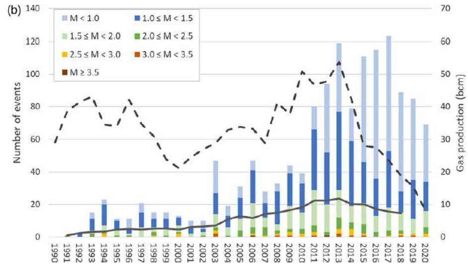
Figure 2-2: (Left) Map of earthquakes recorded by KNMI from 1960-2020, with marker size scaled to magnitude; (Right) Plots of production history (production volume) and numbers of earthquakes during each year from 1990-2020.
