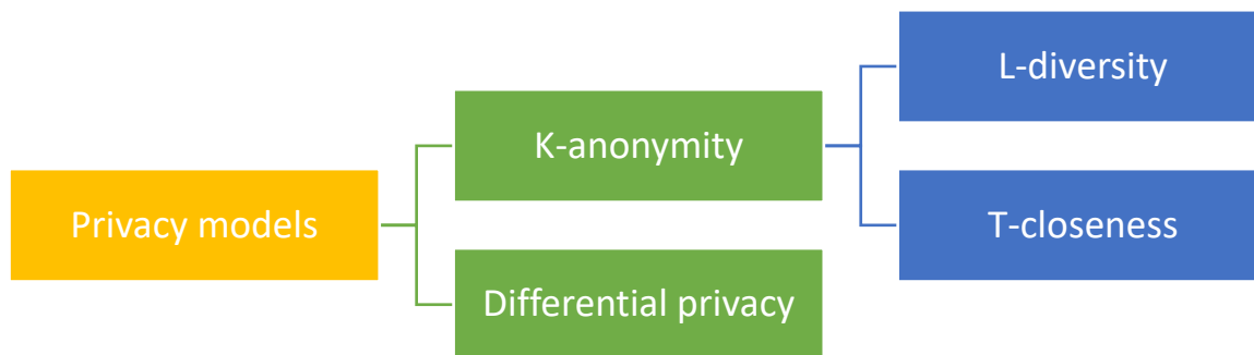
Figure 2: Privacy models
