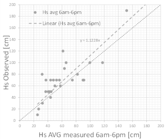
Figure 3.12 - Observed wave height versus measured average wave height during daytime on sailing days.
