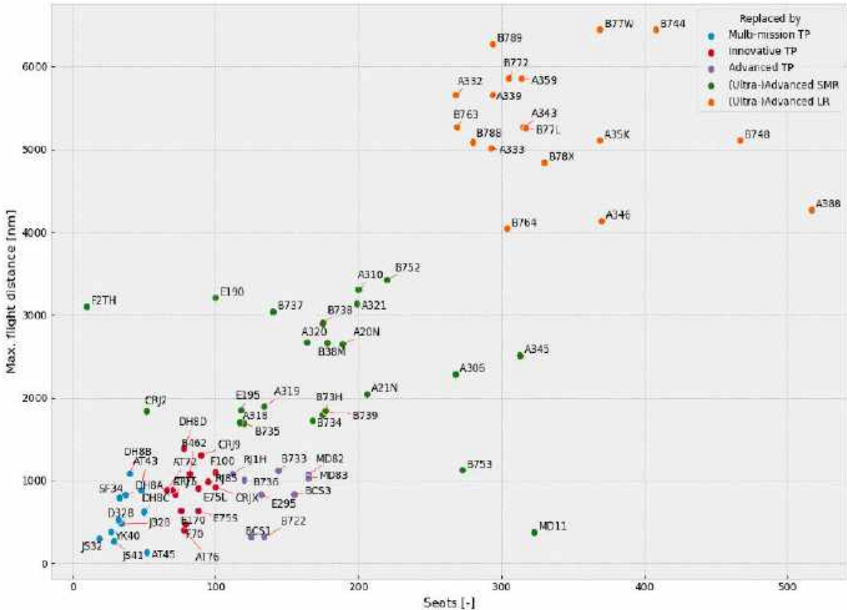
Figure 22: Modelled aircraft replacements based on 2019 aircraft range and seating capacity
