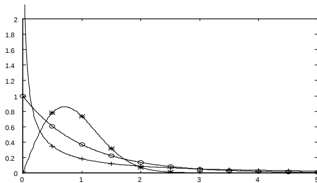
Figure A-1: Weibull function for \eta=1 and (*) \beta=1/2 ; (°) \beta=1 ; (*) \beta=2
