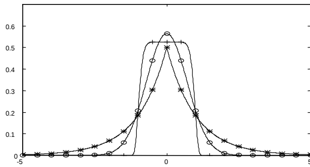
Figure A-2: Generalised-Laplace function for a=1 and (+) b=0,1 ; ( ^{\circ} ) b=\frac{1}{2} ; (*) b=1
