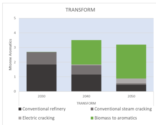
Figure 3.8 - Aromatics production for TRANSFORM scenario (technology selection)
